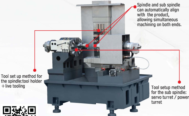
Note: SA45-VS Frame
