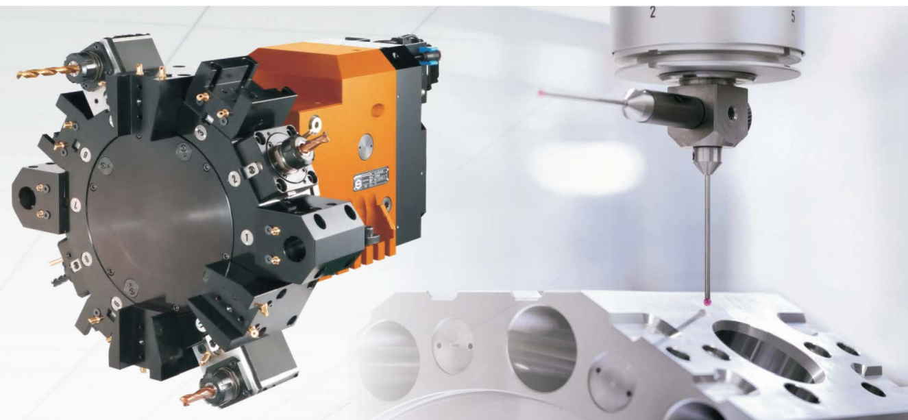
Various VDI Tool Holders
