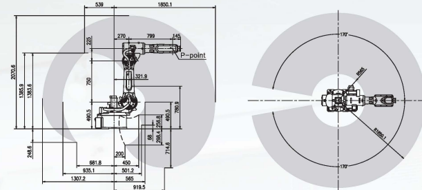
URB35-1850 Motion range diagram
