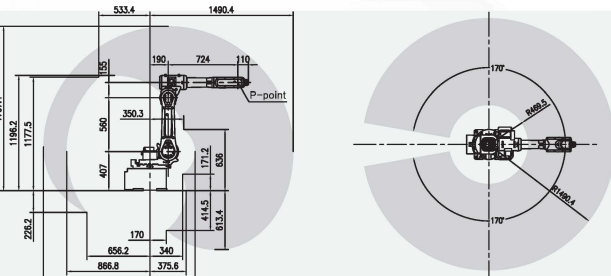
URB08A-1490 Motion range diagram
